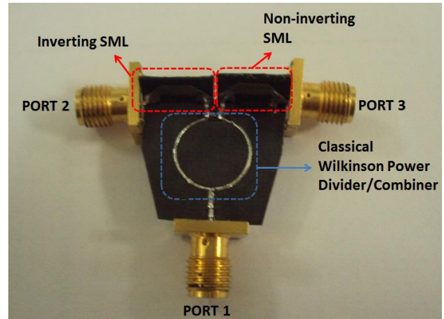
Fig. 2. Fabricated 180^\circ power divider/combiner.
