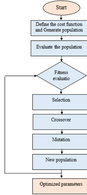
Fig. 2. GA flowchart
