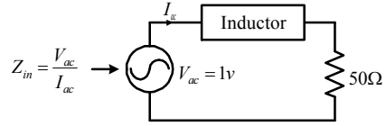
Fig. 12. circuit for FAI simulation
