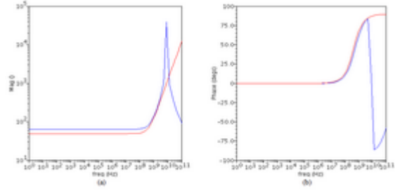
Fig. 13. Floating ideal (red) and active (blue) inductor simulation (a) magnitude (b) phase
