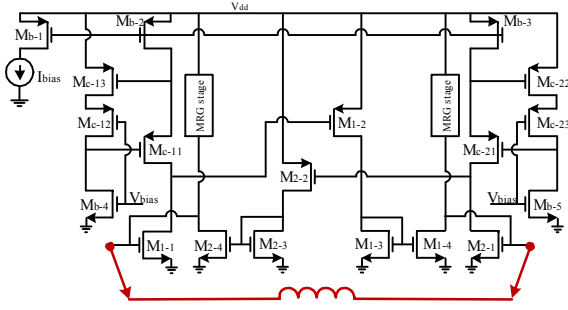
Fig. 9. Circuit implementation of proposed FAI
