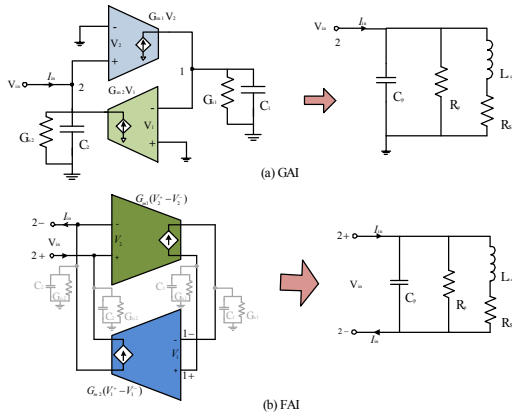
Fig. 4. Block diagram of AI realization by OTA and equalant passive model (a) Grounded (b) Floating
