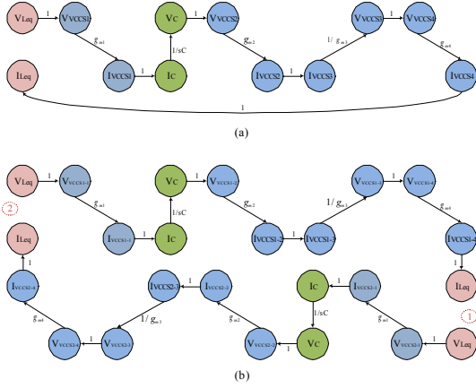
Fig. 3. (a) Modified SFG for Grounded AI. (b) SFG for Floating AI
