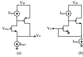
Fig. 6. simplified CMOS-based GAI
