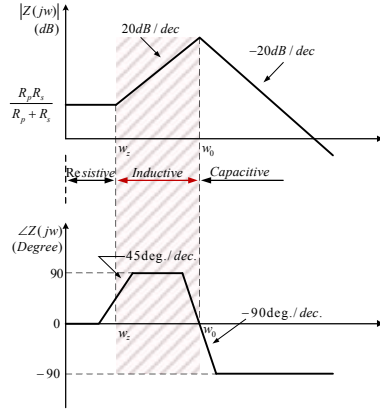
Fig. 5. Bode plots of the impedance of lossy Gyrotor-C AI
