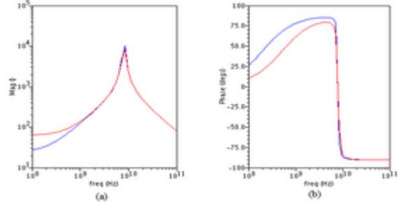
Fig. 11. Compression AI circuits with (blue) and without (red) MRC stage (a) magnitude (b) phase
