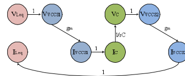
Fig. 2. General SFG for AI's circuit generation with VCCS
