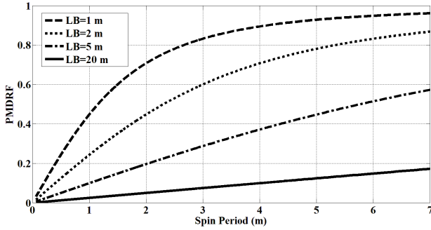
Fig. 2. Evolution of PMDF as a function of spin period for different L_B values
