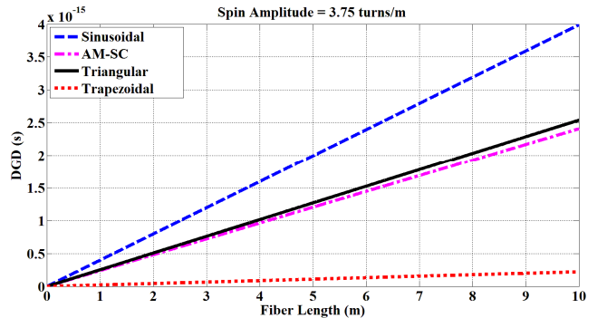
Fig. 7. DGD variation as a function of fiber length \alpha_0=3.75 \text{ turns/m} , p=1 \text{ m} , L_B=5 \text{ m}
