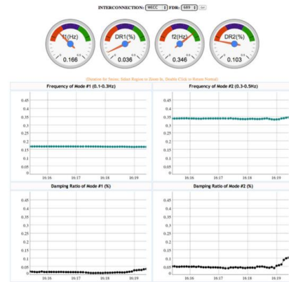
Fig. 7. Online oscillation mode frequency and damping ratio display
