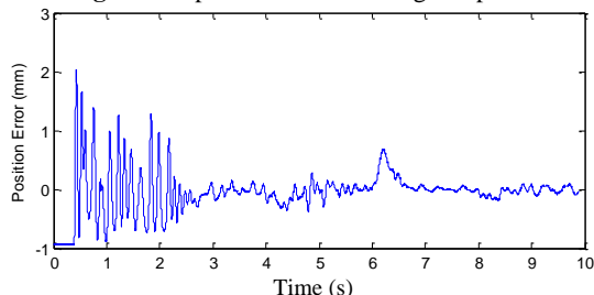
Fig. 12. Experimental position tracking error
