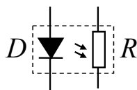
Fig. 1. The optically coupled photoresistor - Vactrol.
