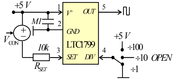
Fig. 16. Connection of voltage controlled oscillator LTC1799
