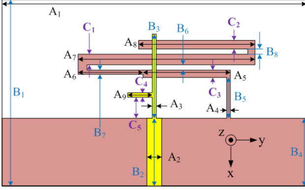
Fig. 1. The antenna geometrical layout and physical parameters
