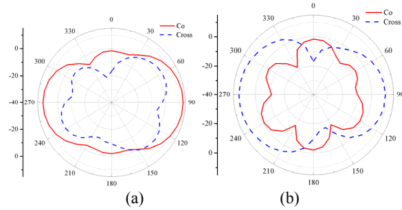
Fig. 8. The measured radiation pattern at 0.7GHz (a) y-z plane and (b) x-z plane
