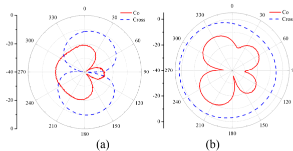
Fig. 9. The measured radiation pattern at 1.5GHz (a) y-z plane and (b) x-z plane
