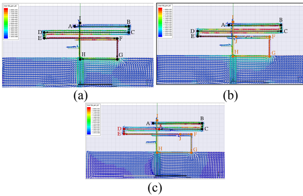
Fig. 4. The simulated surface current distribution at (a) 0.7GHz, (b) 1.5GHz, (c) 1.9GHz
