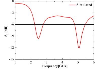
Fig. 2. The simulated S 11 of tree-type monopole
