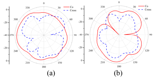
Fig. 12. The measured radiation pattern at 5.2GHz (a) yz plane and (b) xz plane
