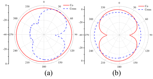
Fig. 11. The measured radiation pattern at 2.4GHz (a) y-z plane and (b) x-z plane
