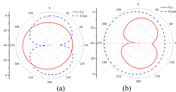
Fig. 10. The simulated radiation pattern at 1.9GHz (a) y-z plane and (b) x-z plane
