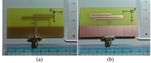
Fig. 6. The fabricated prototype antenna shown in two opposite sides, (a) front view, (b) back view
