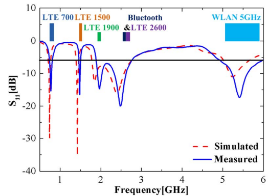
Fig. 7. The measured and simulated antenna S_{11} and the corresponding wireless access standards
