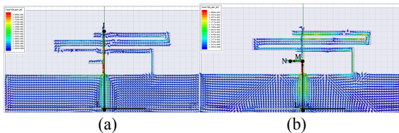
Fig. 5. The simulated surface current distribution at (a) 2.4GHz, (b) 5.2GHz
