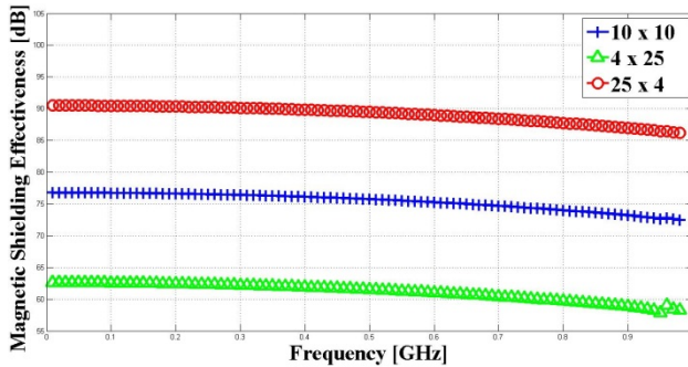
Fig. 6. Theoretical MSE for 160x160x800 mm size enclosure having different aperture shape
