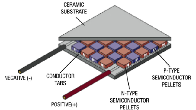
Fig.1 TEG structure
