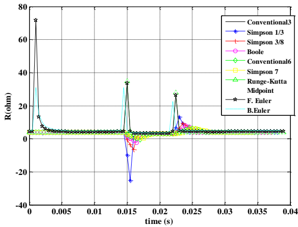
Fig. 2. Not filtered R values calculated before and after the fault
