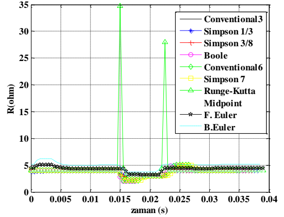
Fig. 4. Filtered R values calculated before and after the fault
