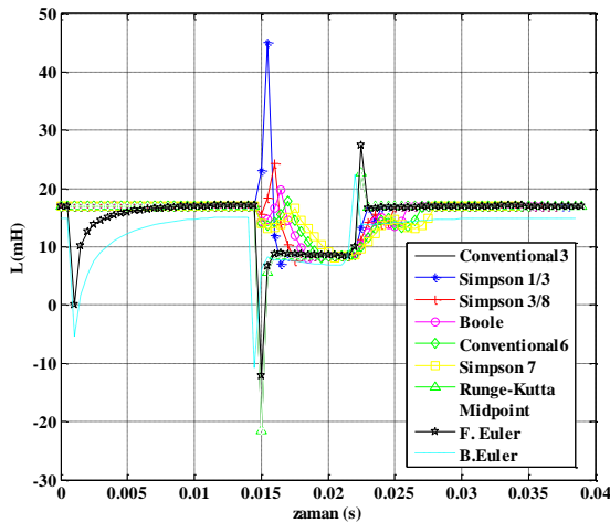
Fig. 3. Not filtered L values calculated before and after the fault
