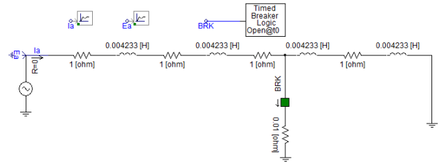
Fig. 1. Single-phase line model
