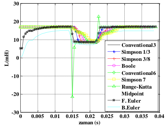
Fig. 5. Filtered L values calculated before and after the fault
