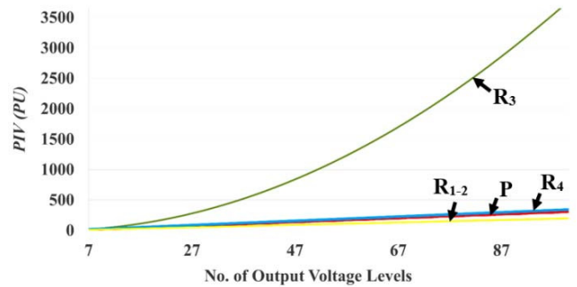
Fig. 7. Total PIV value versus number of levels for proposed topology and other mentioned solutions
