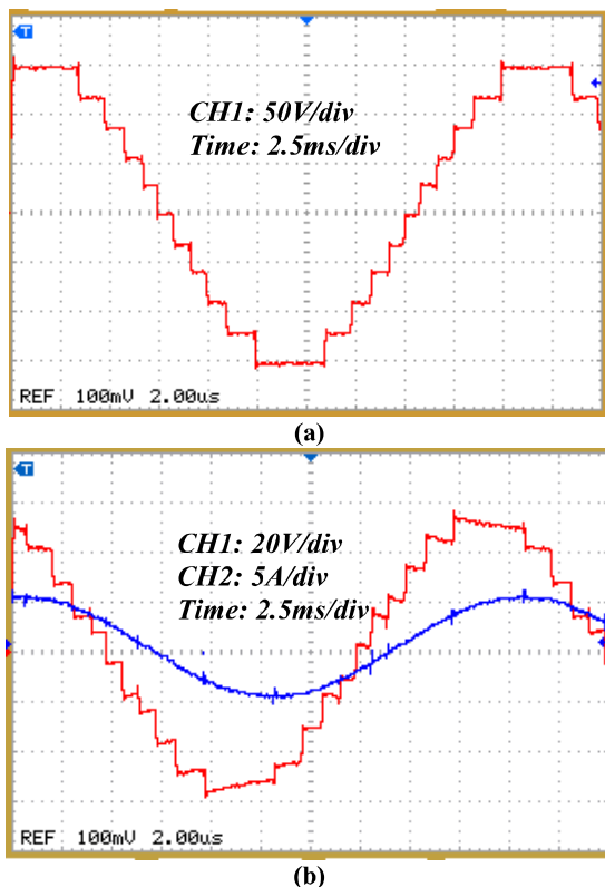
Fig. 10. Experimental results of implemented 11-level proposed inverter
