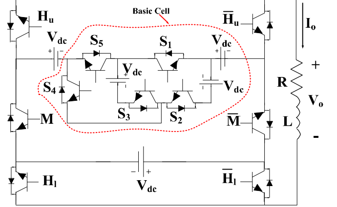
Fig. 8. Circuit diagram of 11-Level multilevel inverter
