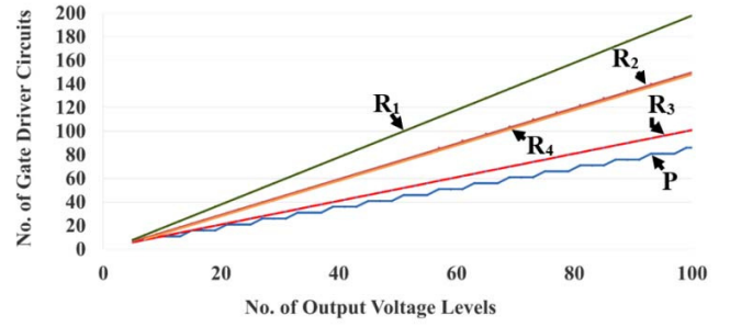
Fig. 5. Number of gate driver circuits versus number of levels for proposed topology and other mentioned solutions
