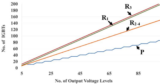
Fig. 4. Number of IGBTs versus number of levels for proposed topology and other mentioned solutions
