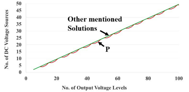
Fig. 6. The number of DC voltage sources versus number of levels for proposed topology and other mentioned solutions
