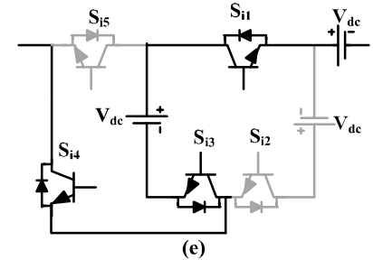
Fig. 1. a) Circuit diagram of the basic cell of proposed MVSI and Equivalent circuits of it for; b) 3V_{dc} , c) 2V_{dc} , d) V_{dc} , and e) zero level
