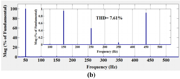
Fig. 9. a) Voltage and current waveforms and b) harmonics content of voltage of the proposed 11-level inverter
