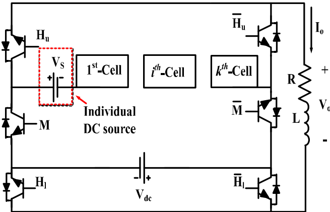
Fig. 2. Proposed MVSI
