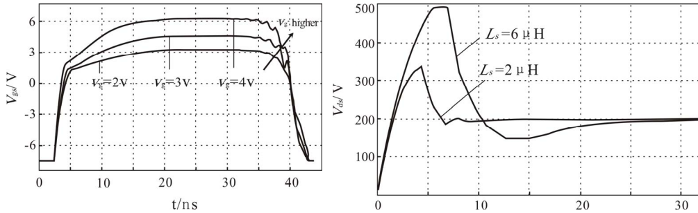
(a) Influence of driving source v_g (b) Influence of stray inductance L_s FIGURE.6 Switching characteristics of the GaN HEMT model in different conditions
