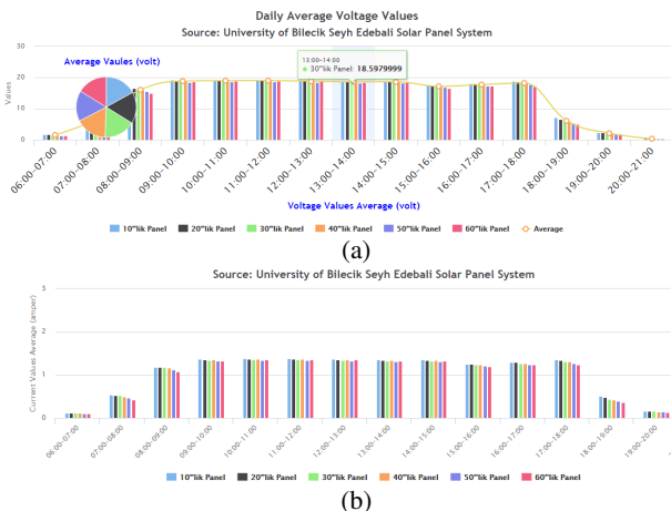
Fig. 10. The daily values of each panel (a) voltage (b) current
