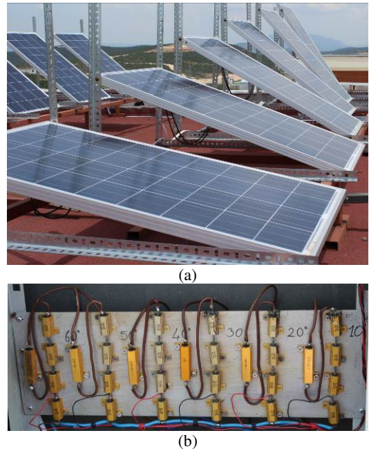
Fig. 7. Experimental setup (a) PV Panels (b) Loads
