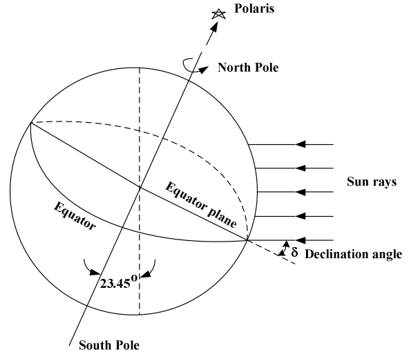
Fig. 1. Declination angle
