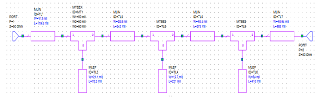
Fig. 7. Schematic representation of the designed 7 th order Gaussian low-pass filter
