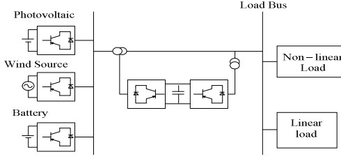
Fig.1 Single-phase microgrid with UPQC
