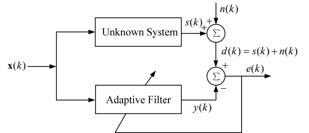
Fig. 2. Block diagram of a system identification problem
