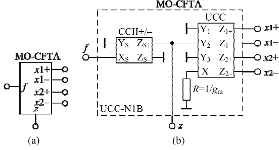
Figure 2. (a) Circuit symbol of MO-CFTA, (b) its implementation using UCC-N1B.
