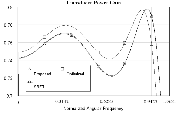
Fig. 5. Closer examination of the gain performances
