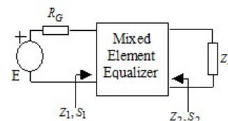
Fig. 1. Single matching arrangement
